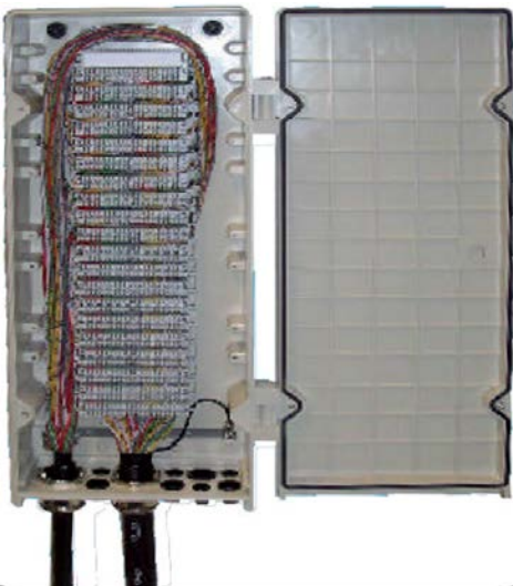
Outdoor Distribution box – 200 pairs (picture is not equal to the shipment)
